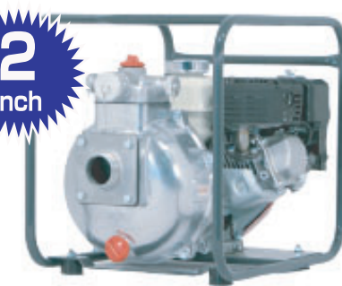
QP-205SX (HONDA GX160) Max Head: 90m Max Flow: 350ℓ/min
